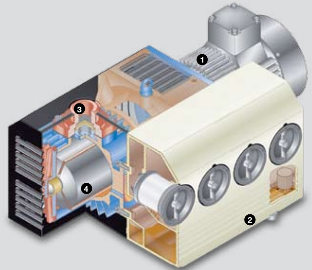
1 Motor | 2 Oil separation | 3 Suction port | 4 Cylinder
