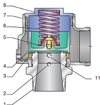
Model 215V
