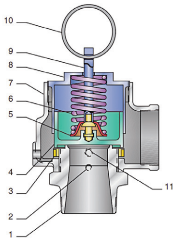
Model 337
