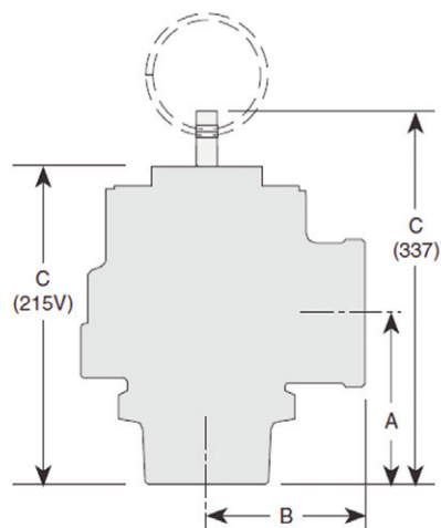
Model 337
